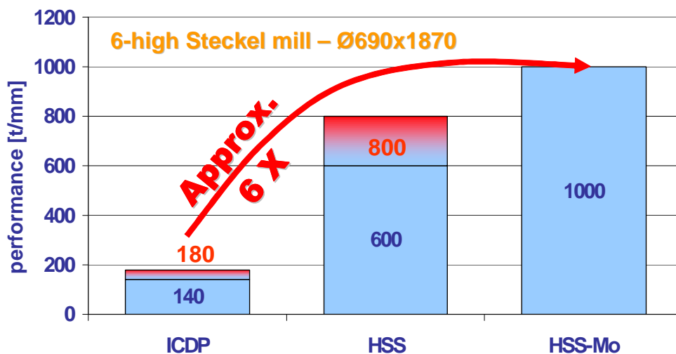
Figure 11: increase in performance by changing the roll system in a 6-high Steckel mill
