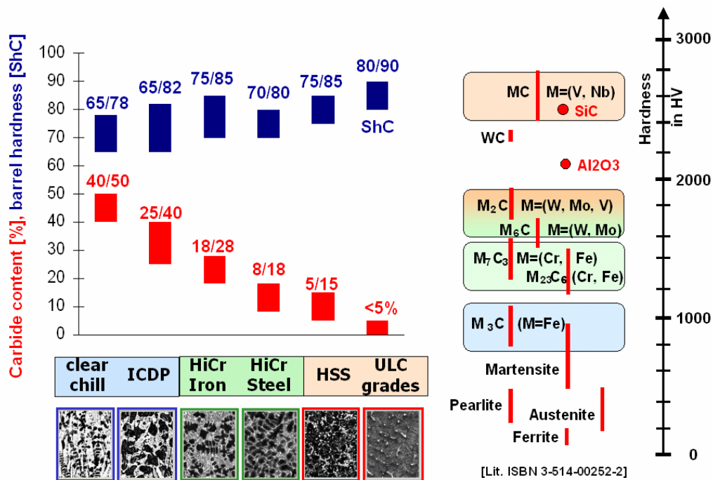
Figure 3: roll grades for hot rolling of flat products [2, 3]
