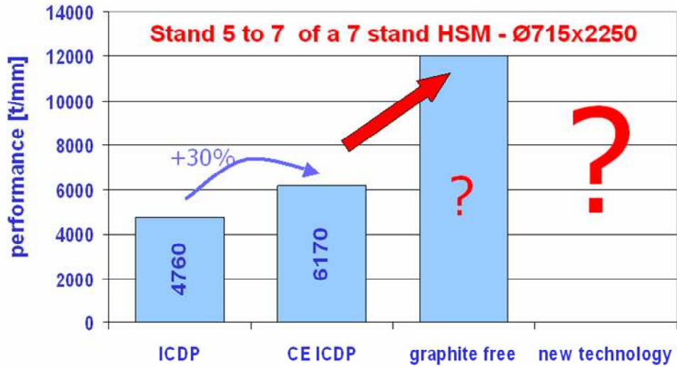
Figure 9: increase in performance by changing the roll system in stand F5 - F7 of a 7 stands hot strip mill
