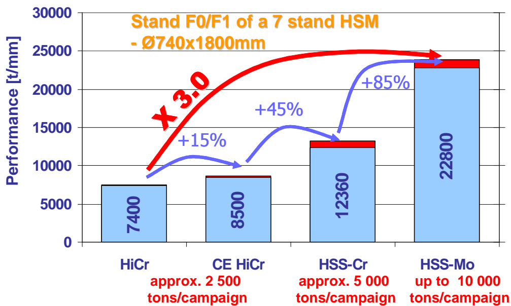
Figure 7: increase in performance by changing the roll system in stand F2 of a 7 stands hot strip mill
