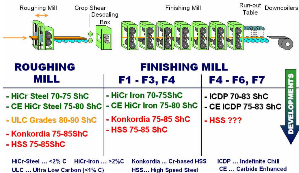
Figure 1: work roll types for hot rolling of flat products
