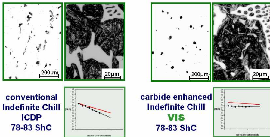
Figure 10: comparison of shell microstructure and hardness drop of conventional ICDP and carbide enhanced Indefinite (VIS) [6]
