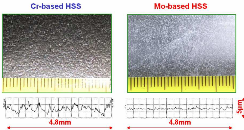
Figure 8: barrel surface after rolling 3 000 tons in stand F2 of a 7 stands hot strip mill (Ø820x2350) [5]
