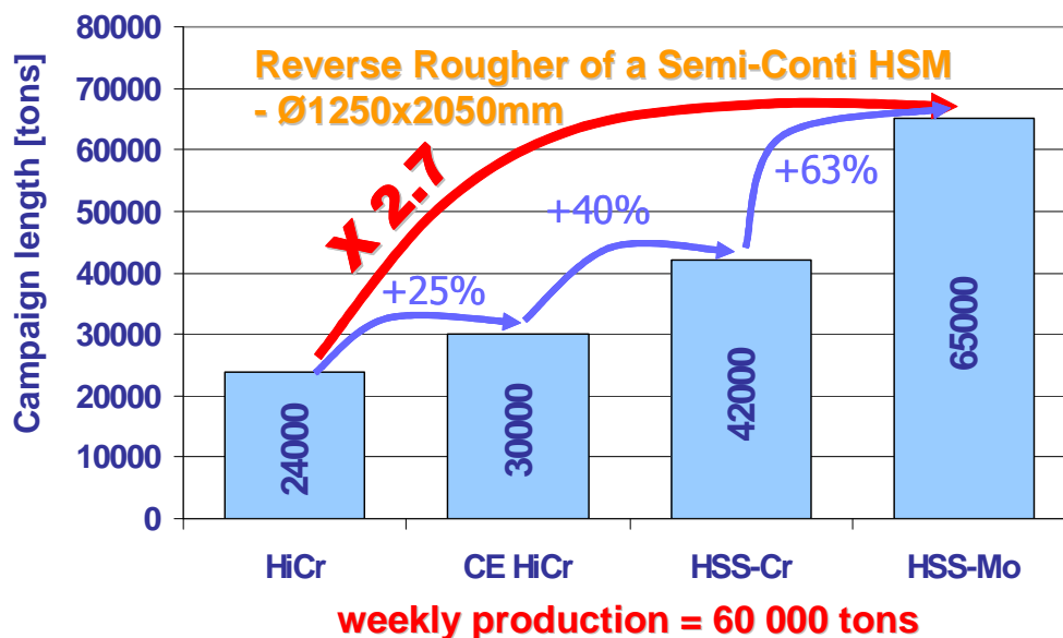
Figure 4: increase in campaign length by changing the roll system in a single reversing roughing stand of a semi-continuous hot strip mill
